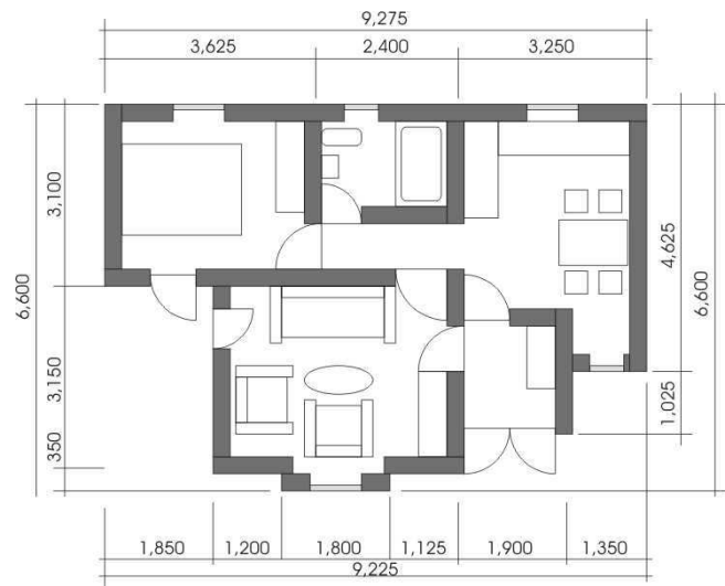
Figure 7. Floor plan of the analyzed example
