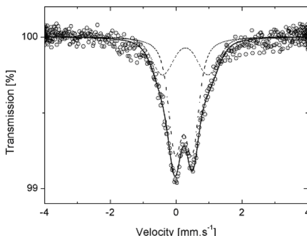
Figure 1 Mössbauer spectrum of the natural bentonite Slika 1. Mössbauerov spektar prirodnih bentonita
