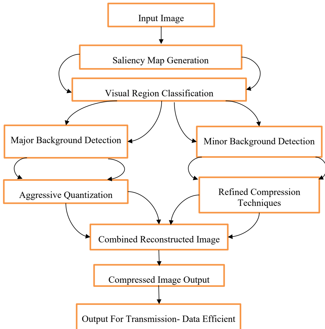
Figure 1. Hierarchical image compression pipeline with saliency-based classification and reconstruction
