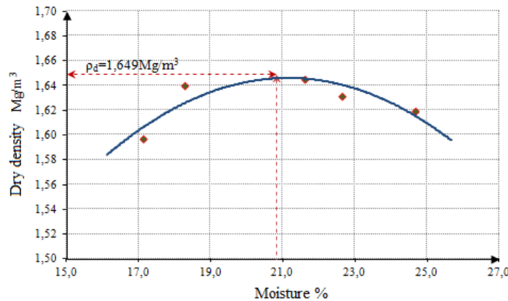
Figure 3 Compaction characteristics Proctor test
