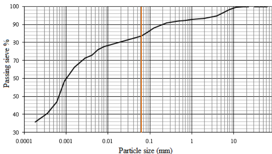
Figure 2 Granulometry diagram
