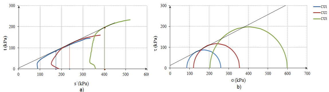
Figure 8 a) Shear illustrated by stress path, b) Shear strength diagram
