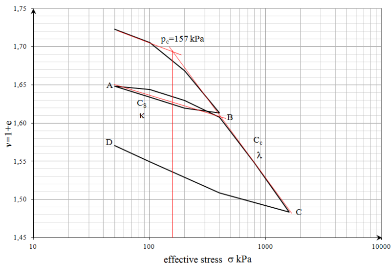
Figure 4 Specific volume v /effective pressure \sigma ratio
