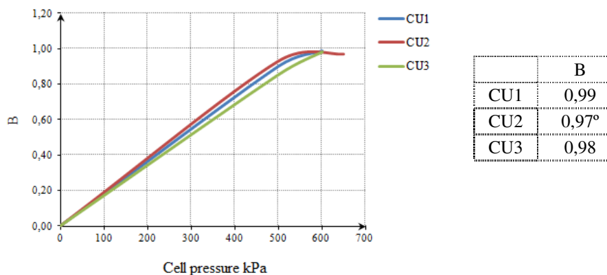
Figure 5 Saturation phase CU test
