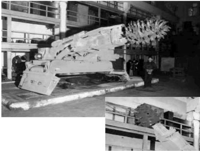
Figure 2. Remotely controlled support-walking roadheader (model KPA-3M)
