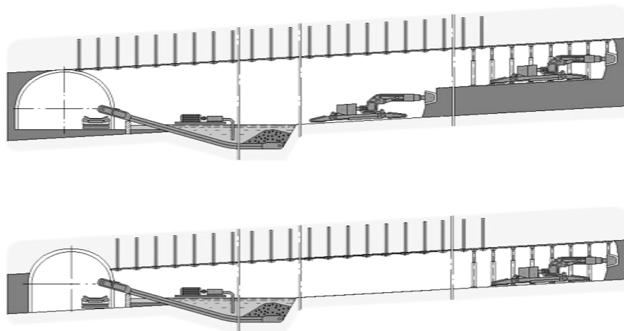
Figure 3. Continuous driving (drifts) technology by mechanical-hydraulic support-walking
